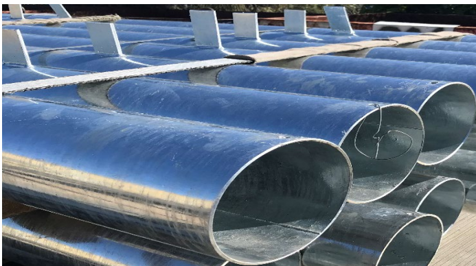
Hot Dip Galvanised is a much cleaner finish
